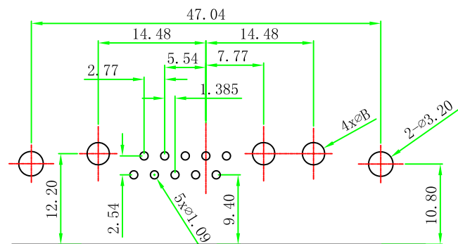
PCB LAYOUT
