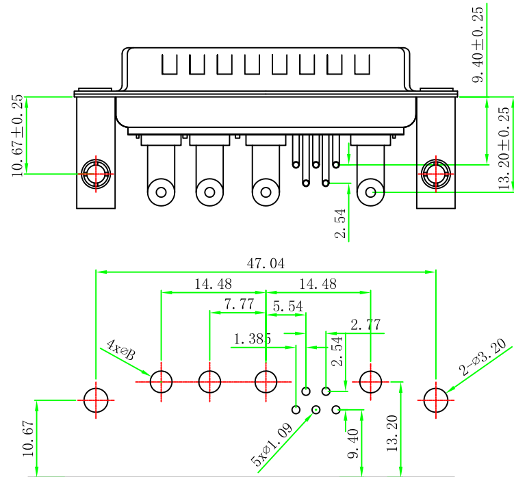
PCB LAYOUT
